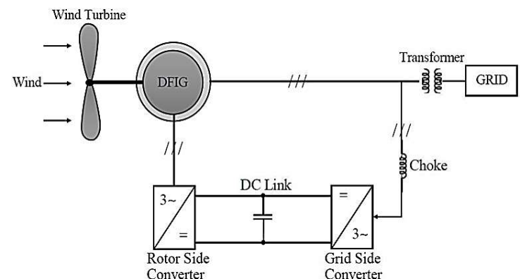
Fig. 1: Schematic diagram of DFIG-based wind energy systems. [6]
