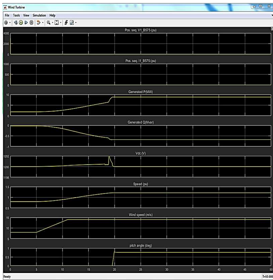
Fig. 3: Simulation result of Wind Farm connected to the Distribution network in Var regulation mode.
