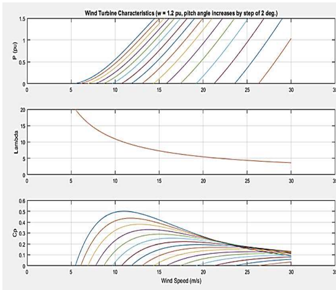
Fig. 5: Plot of Output power (pu), Tip Speed – Ratio( \lambda ) and Power Coefficient( C_p ) against Wind Speed (m/s).
