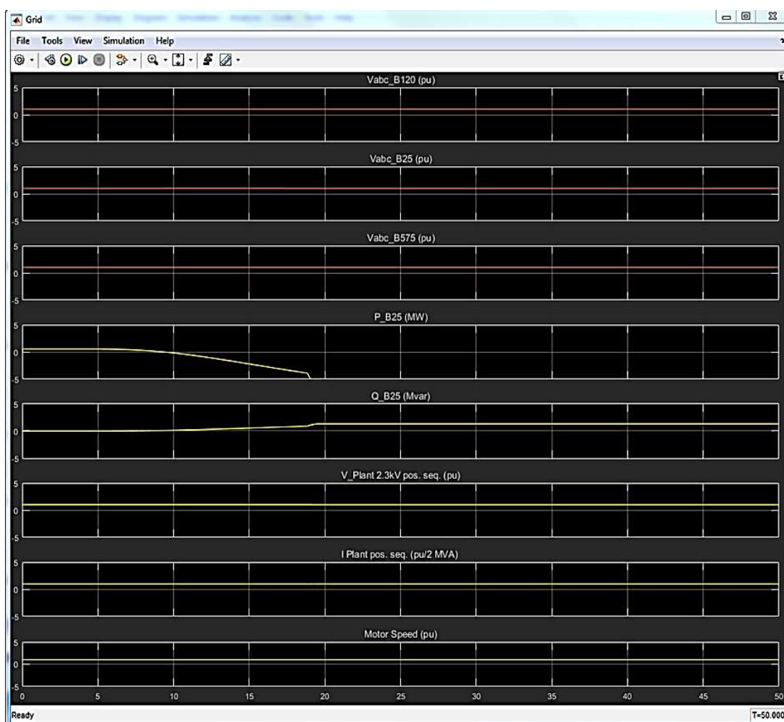
Fig. 4: Simulation result of Wind Farm connected to the Distribution network with short circuit fault at 10km from the grid.
