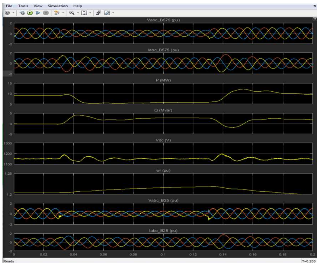
Fig 2: Simulation result for the wind farm when the wind speed is 15m/s
