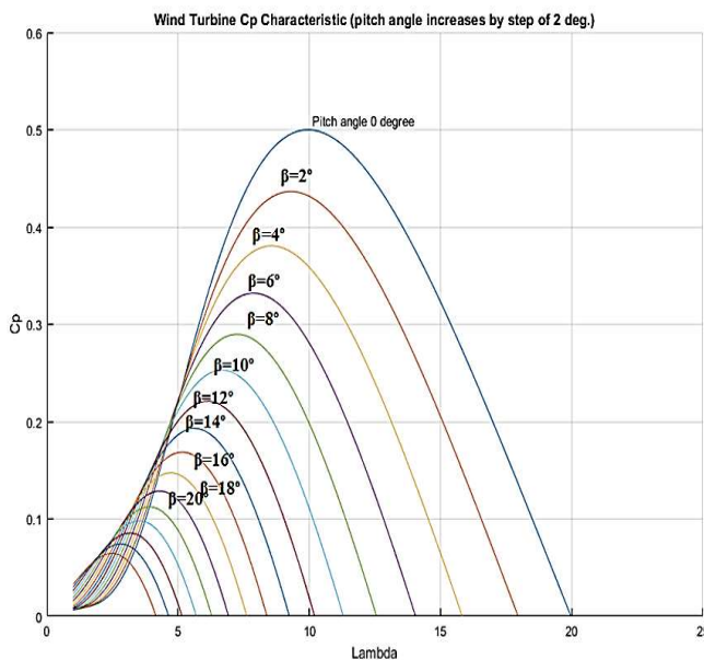
Fig. 6: Wind Turbine Power Coefficient Characteristics plot
